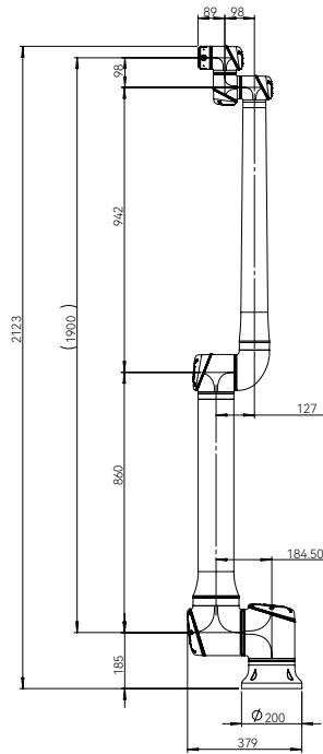
EC64-19 external dimensional drawing
