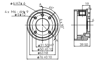
EC64-19 end flange
